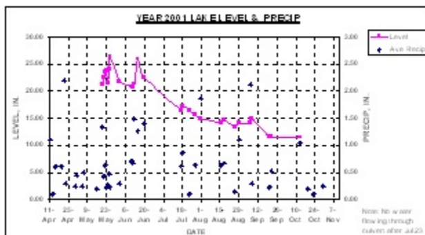
Figure 6. Lake levels and precipitation for the Pipe Lakes.
