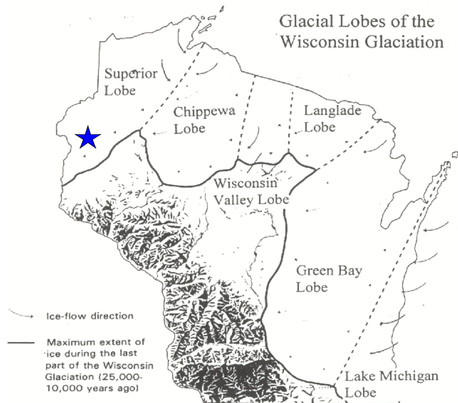
Figure 2. Glacial lobes of the Wisconsin glaciation. The Pipe Lakes are located in the Superior lobe.
