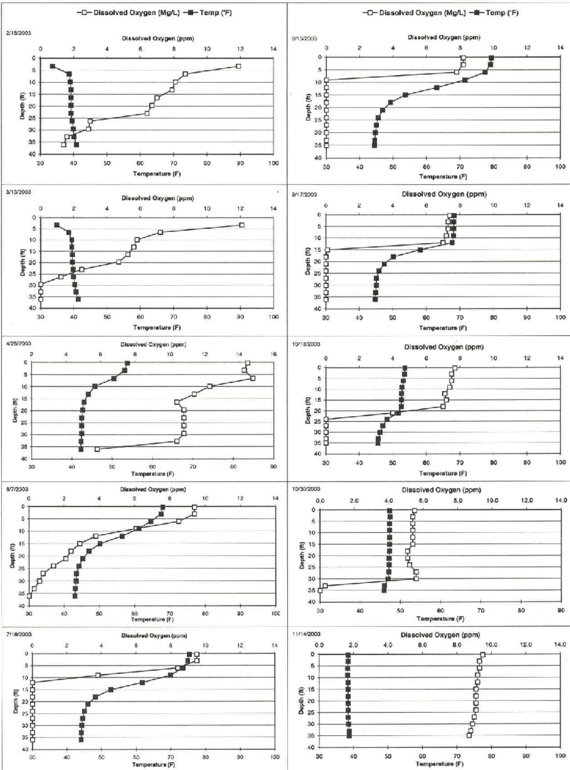
North Pipe Lake - 2003 Dissolved Oxygen and Temperature Profiles
