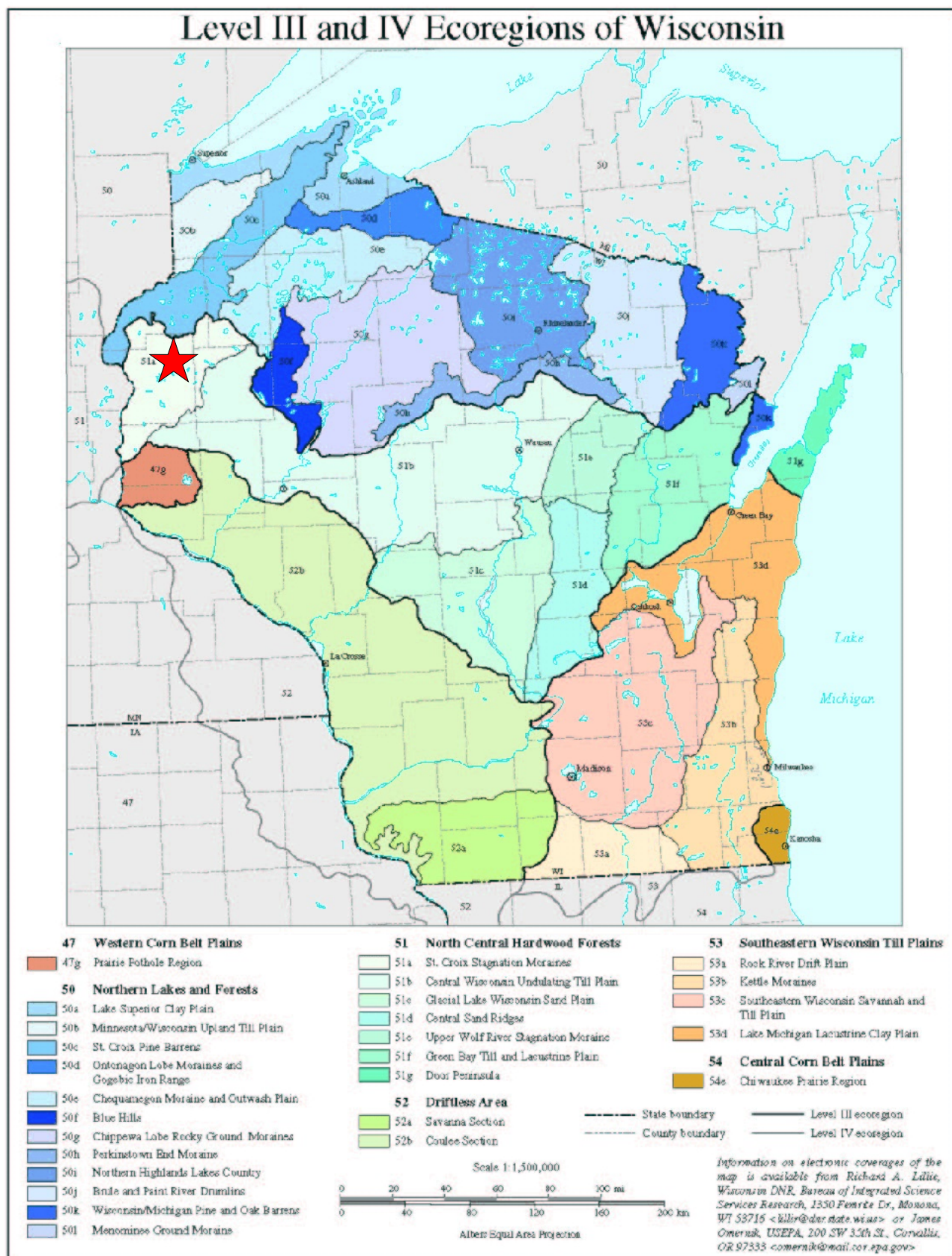
Figure 23. Ecoregion map for Wisconsin. Areas that are labeled with a “50” are within the Northern Lakes and Forest Ecoregion. Areas labeled with a “51” are in the North Central Hardwood Forest Ecoregion. The Pipe Lakes, located in central Polk County are officially in the North Central Hardwood Forest Ecoregion but close to the Northern Lakes and Forest Ecoregion.
