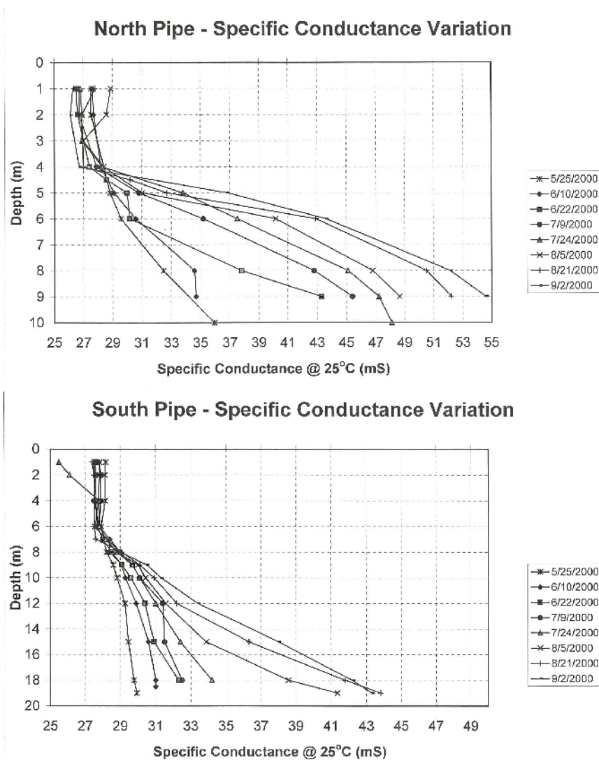
Figure 21. Specific conductance measured for North Pipe and Pipe Lakes in 2000.
